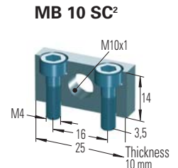
Mounting Block
