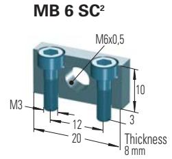
Mounting Block
