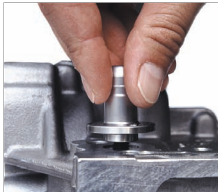
Direct mounting of workpieces - the clamping nipples are mounted directly into the workpiece to be processed
