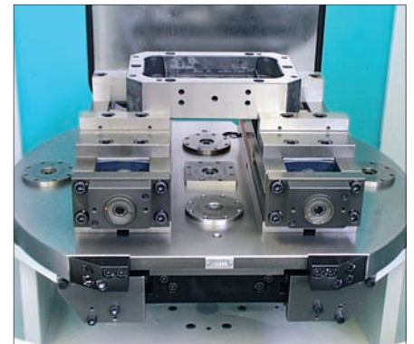
Customized quick clamping pallets with square SPEEDY classic to mount single workpieces
