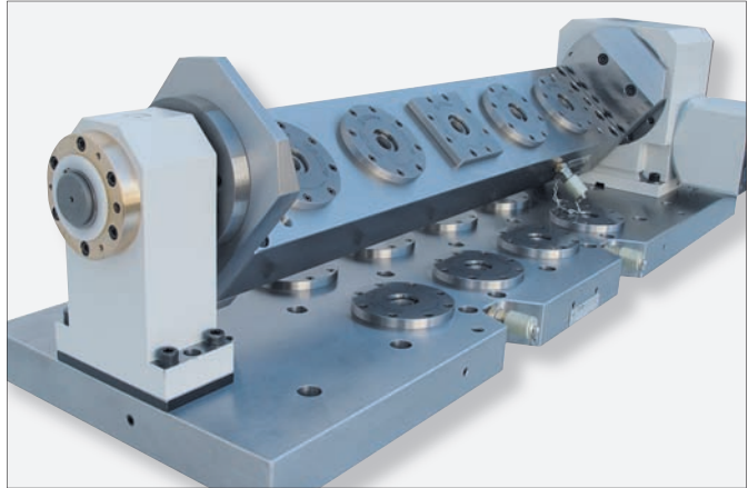
Variable, removable clamping bridge for batch, large and small parts
