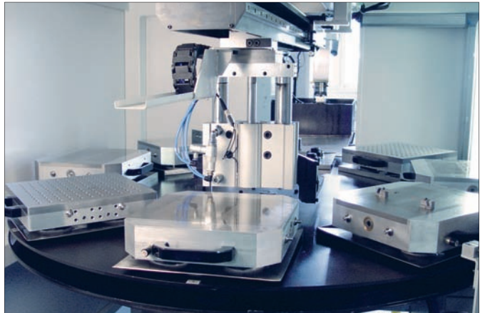
Pallet changer SPW - for automation, can be added to any CNC machining center
