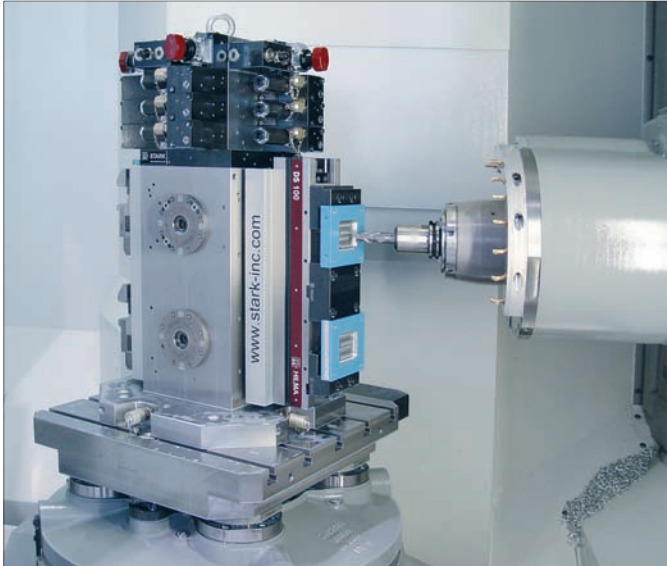
Clamping tower loaded with SPEEDY classic and couplings with blow off and integrated surface control systems
