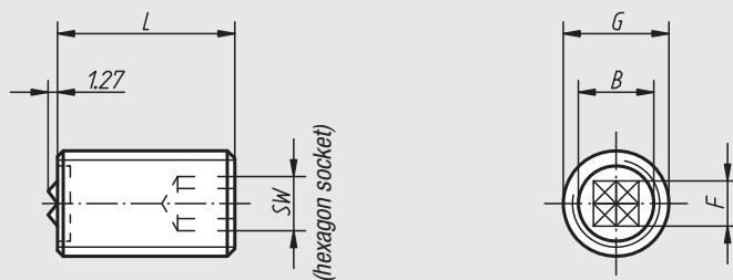
Form C 4-point-serration in hard metal
