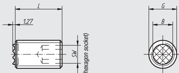
Form B serration in hard metal
