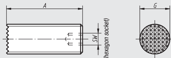
Form A tool steel
